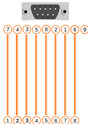
ADAPT RJ45-DB9
