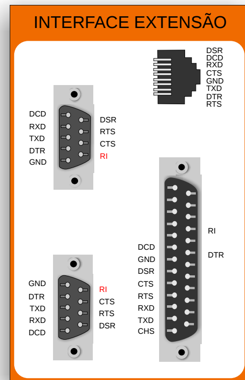
ADAPT RJ45-DB9
